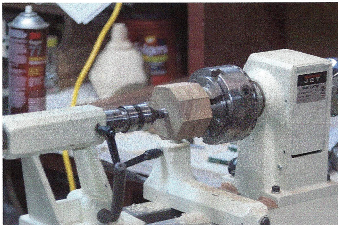
Step 1: Mount block between chuck and live center
