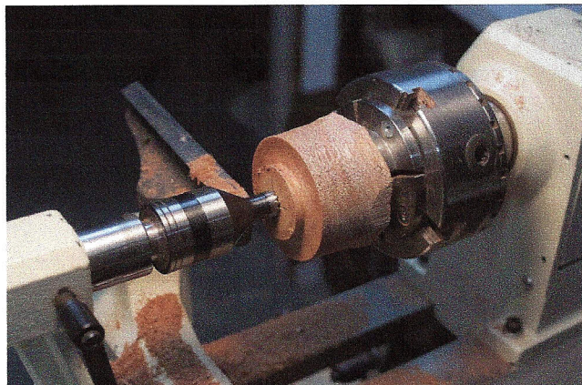
Step 2: Turn a spigot to fit the chuck
