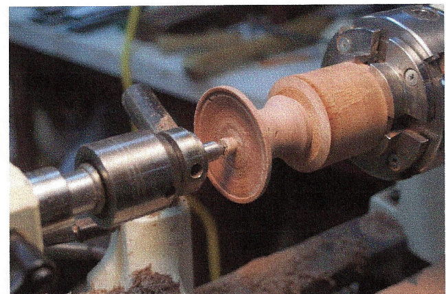
Step 6 install the base on the jam chuck and finish the bottom. The small knob left can be sanded away.
