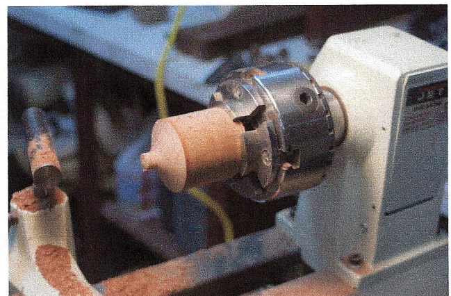
Step 5: Install a block in the chuck and turn a 1/2 inch spigot to accept the base
